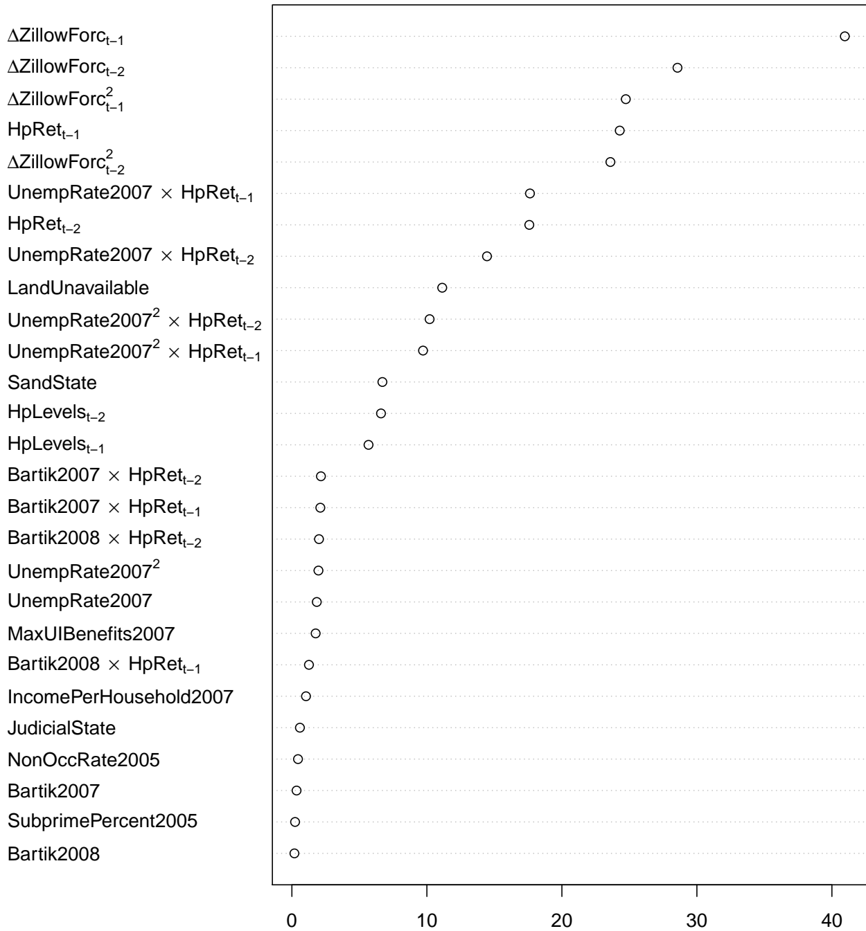
Random Forest Variable Importance -- %IncMSE
